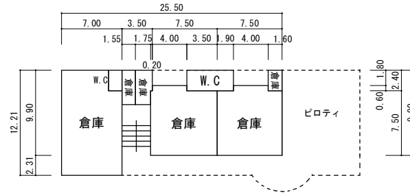
1F
